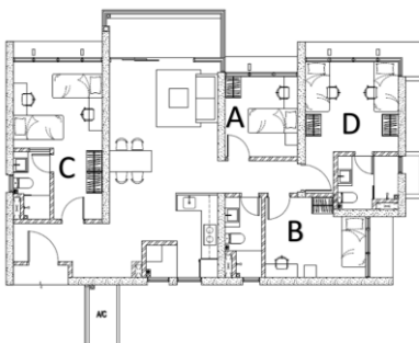
LAYOUT – TYPE G ECO NEST
