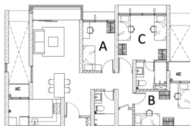
LAYOUT – TYPE E ECO NEST
